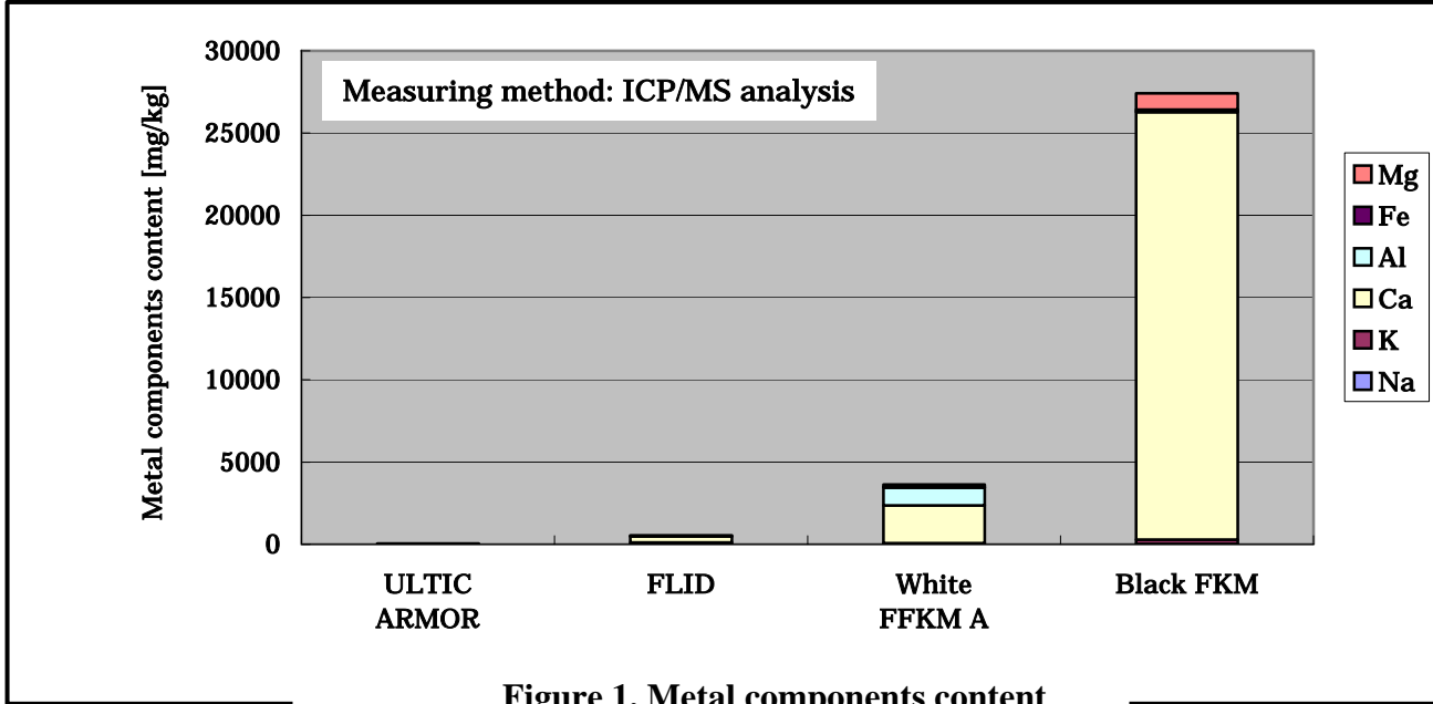
Figure 1. Metal components content
