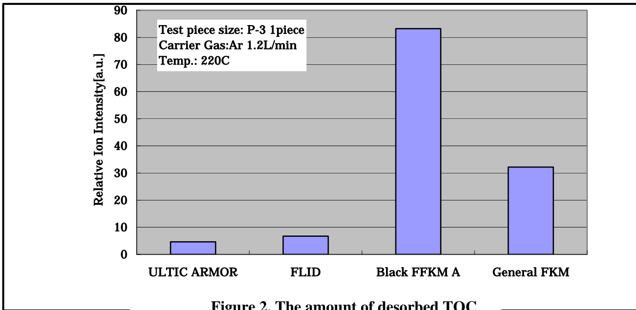
Figure 2. The amount of desorbed TOC
